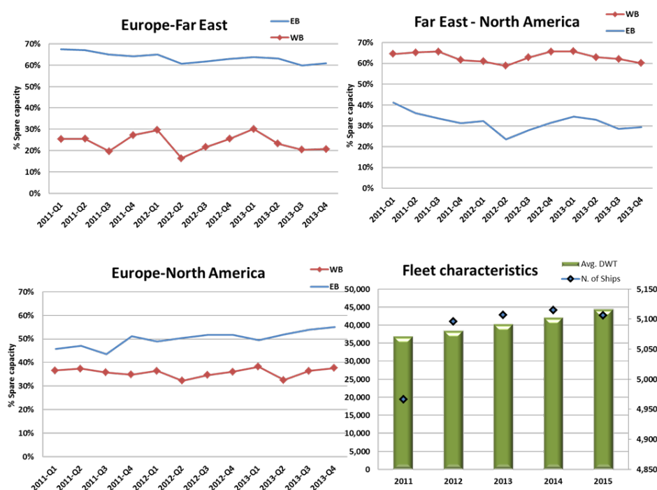
Fig. 10 – Spare capacity on main routes
